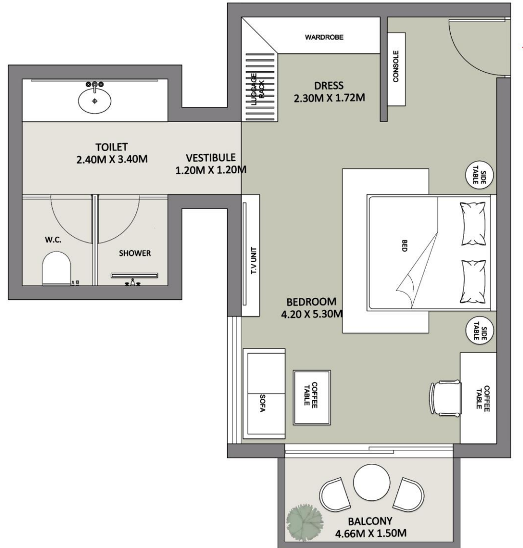
FIRST FLOOR PLAN 540.6 SQ. FT.
